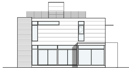
ELEVATION C
